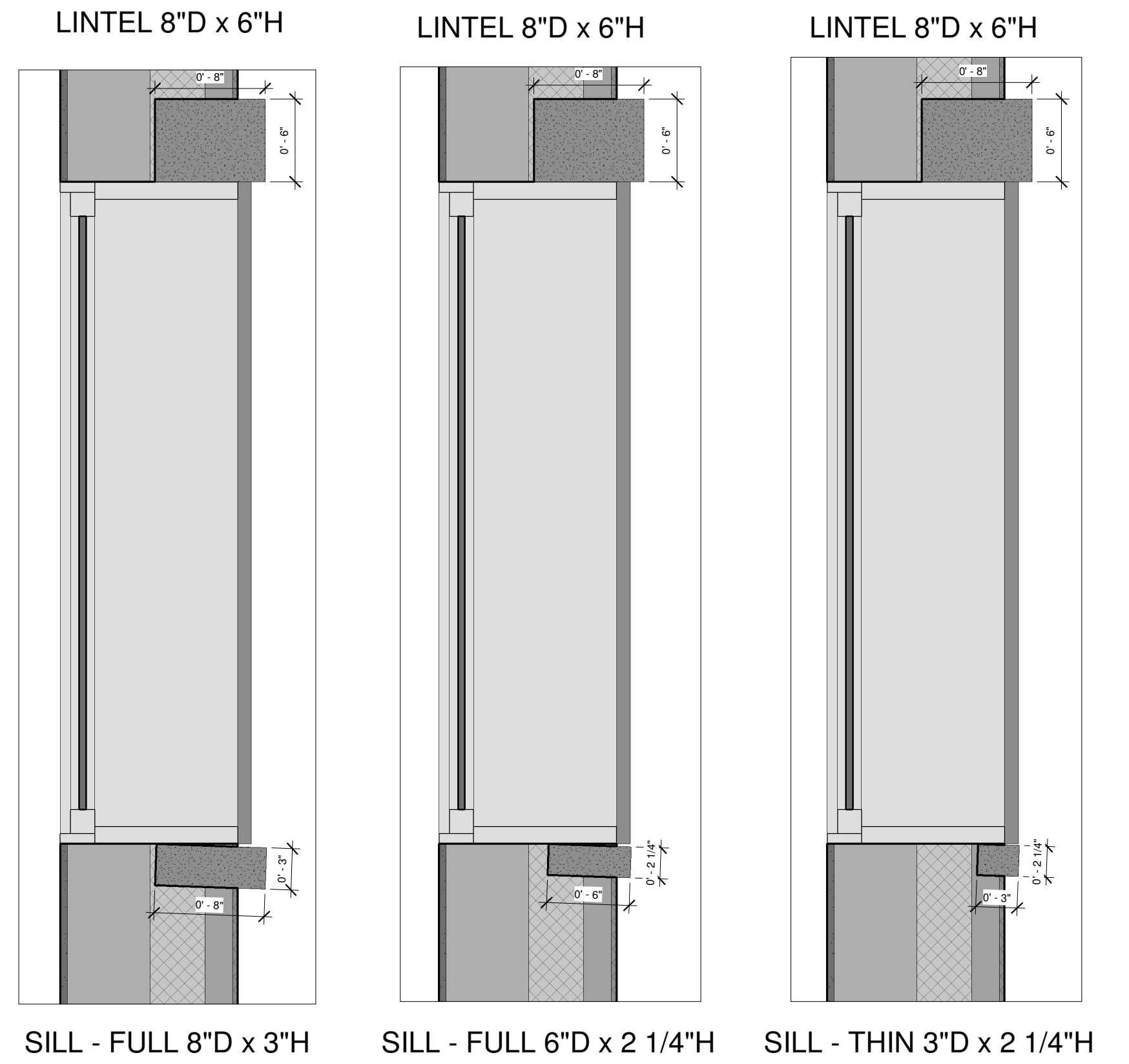
WALL SECTION VIEWS
