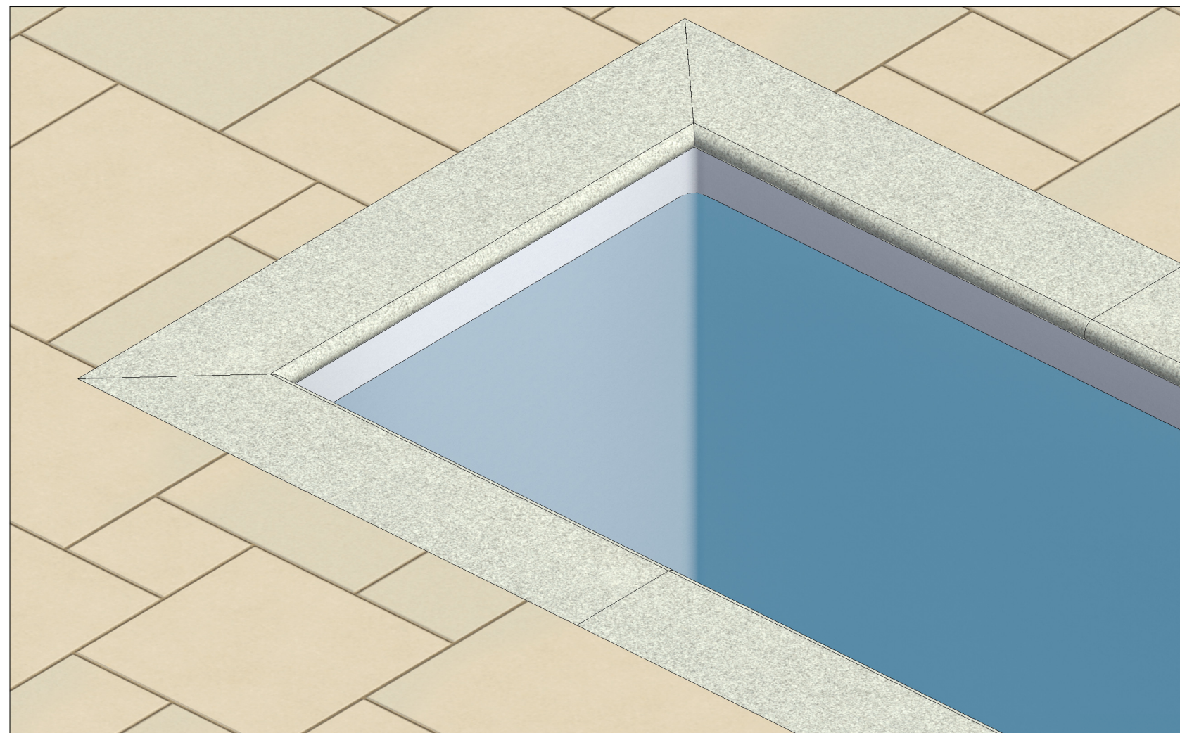
POOL COPING - BULL-NOSED EDGE - 13 1/8" WIDE x 2 1/4" THICK EASTERN GRAY GRANITE™ STONE SHOWN POOL SLAB - INDIANA LIMESTONE™ - BILTMORE PATTERN
