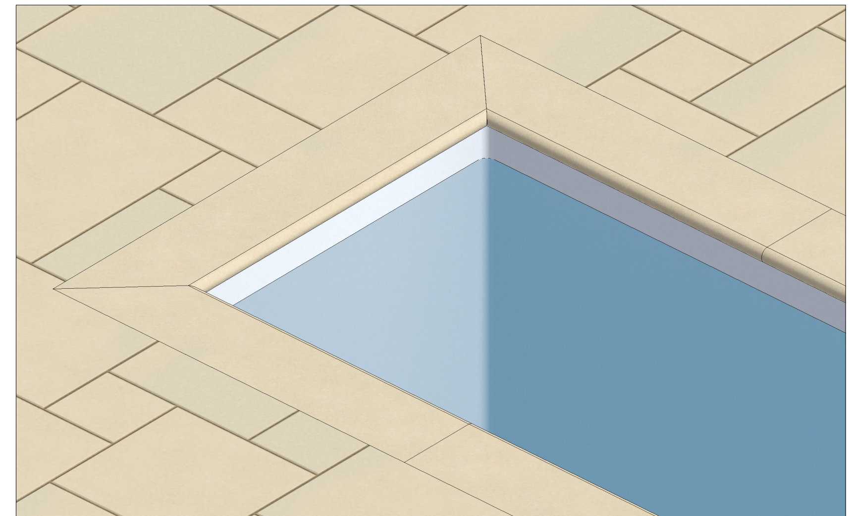
POOL COPING - BULL-NOSE EDGED - 13 1/8" WIDE x 2 1/4" THICK INDIANA LIMESTONE - FULL COLOR BLEND™ STONE SHOWN POOL SLAB - INDIANA LIMESTONE™ - BILTMORE PATTERN
