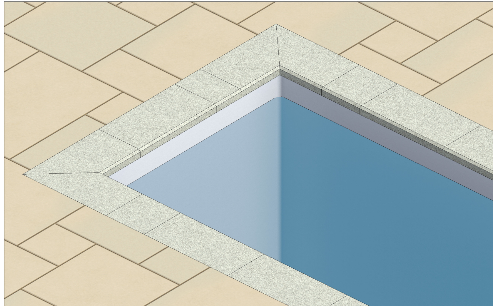
POOL COPING - CHAMFERED EDGE - 12" x 24" x 2" EASTERN GRAY GRANITE™ STONE SHOWN POOL SLAB - INDIANA LIMESTONE™ - BILTMORE PATTERN
