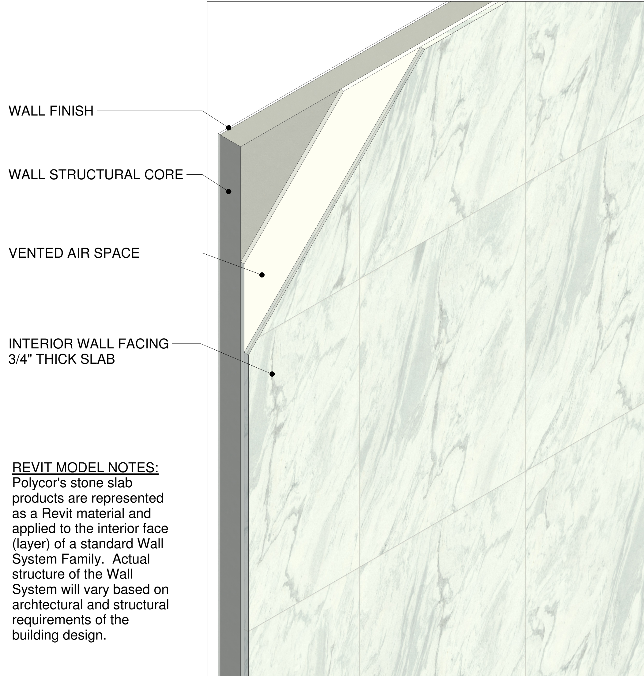
TYPICAL INTERIOR WALL STRUCTURE
