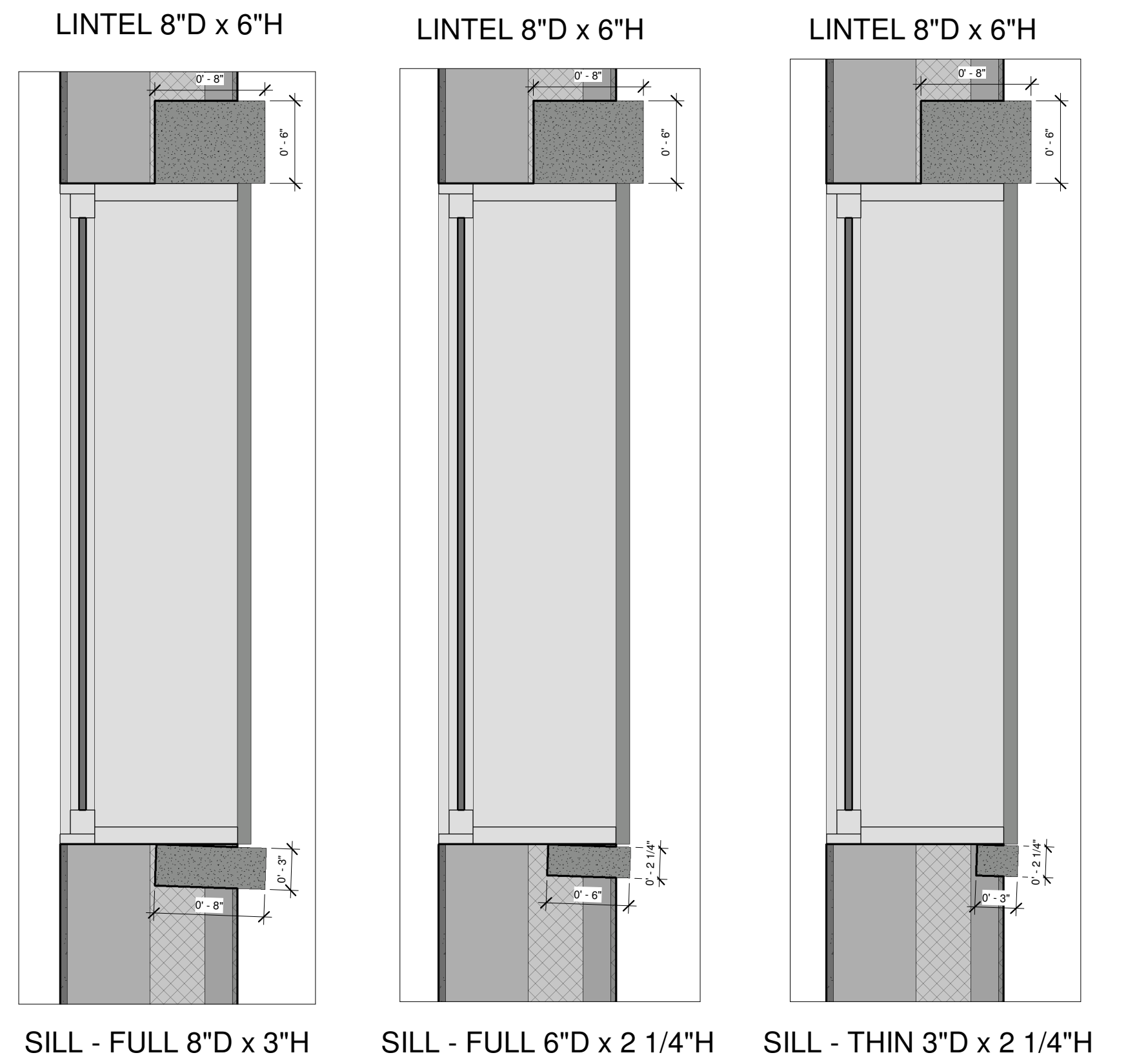
WALL SECTION VIEWS
