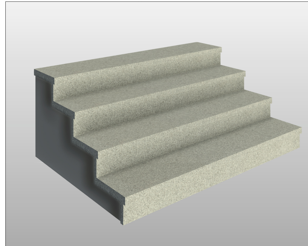
TREAD - 72" x 14" x 2" RISER - 72" x 5" x 1 1/4" INDIVIDUALLY PLACED BARRE GRAY™ GRANITE
